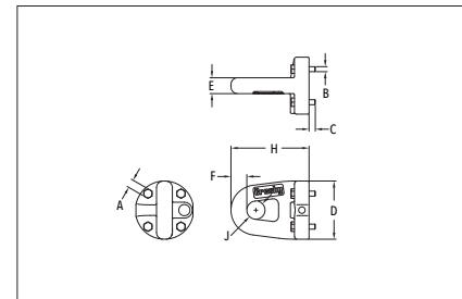
“Eye” Handle
