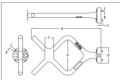
“F” Handle
